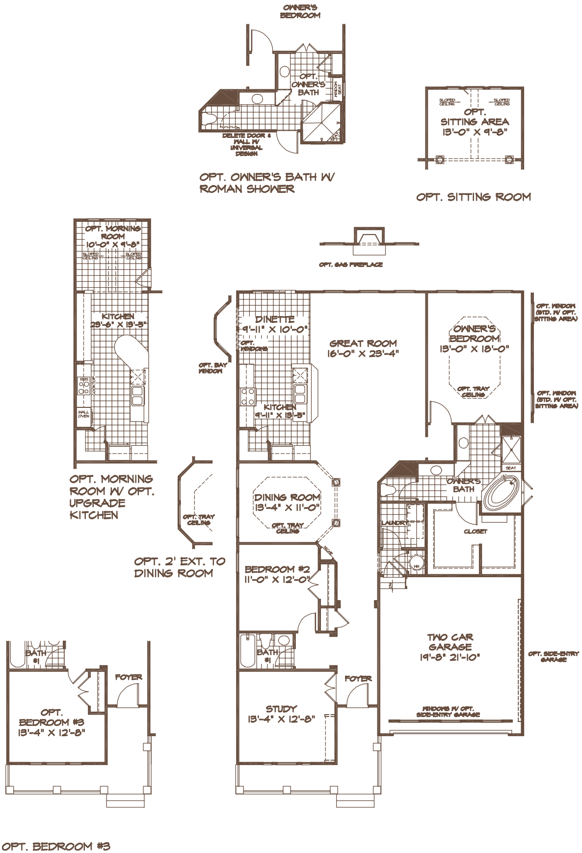
Elevation C
